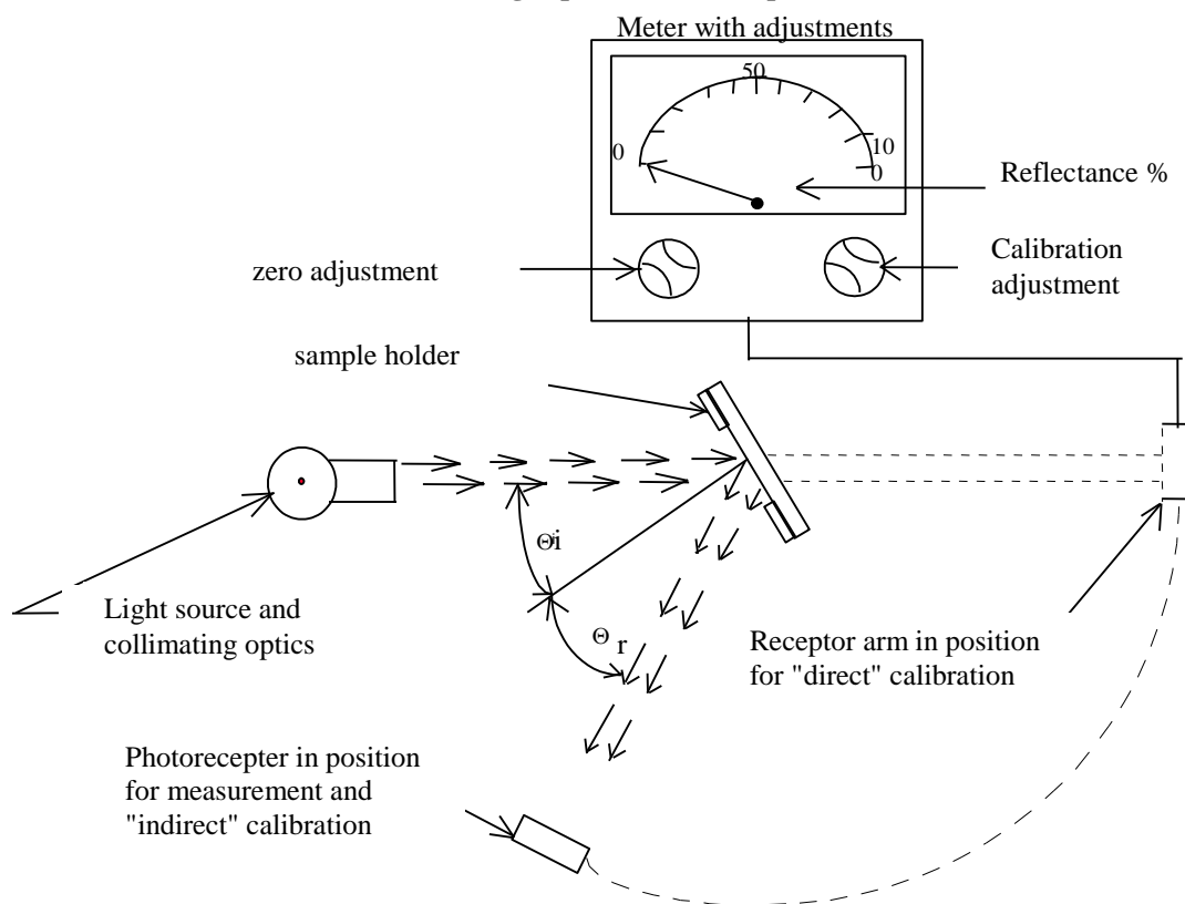
Generalised reflectometer showing experimental set-ups for the two calibration methods
